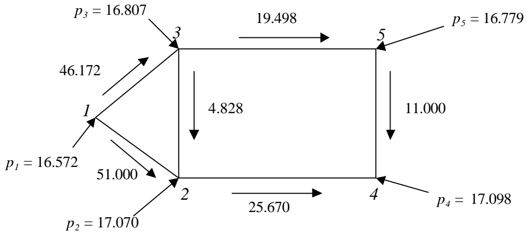
Figure 2: Constrained Dispatch: C_{12}=51, C_{45}=11
