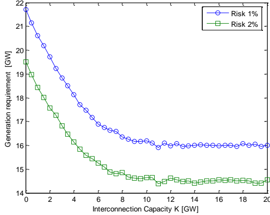
Fig. 4. Generation requirement for a risk of 1% or 2%
