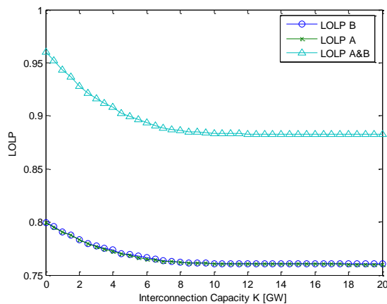
Fig. 3. Lost of Load Probability (LOLP A, LOLP B and LOLP A&B) vs. transmission capacity K
