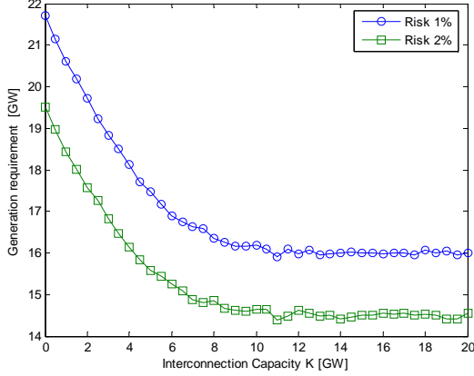
Fig. 4. Generation requirement for a risk of 1% or 2%
