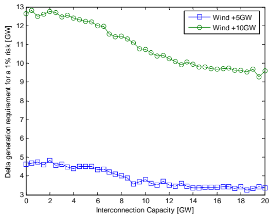
Fig. 8. Difference between generation requirement for a risk of 1% with wind and without wind corresponding to zone B
